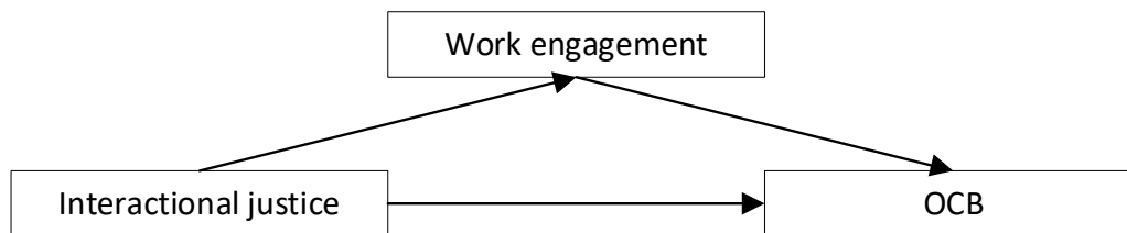
Fig. 1: Research model
