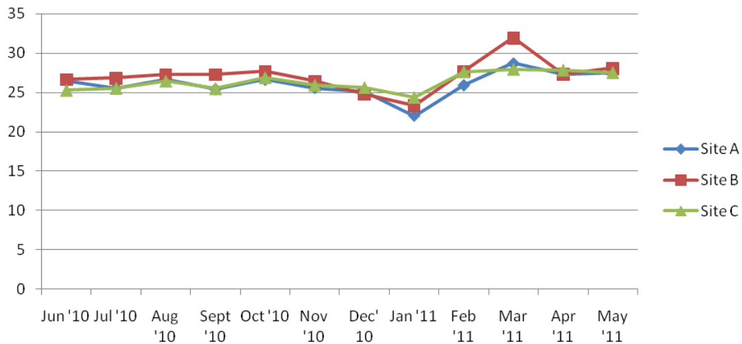
Fig. 2. Monthly Variation of Temperature across the Sampling sites in Lower River Benue
