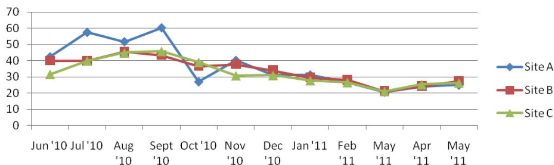
Fig. 6: Monthly Variation of Total Dissolved Solids across the Sampling sites in Lower River Benue
