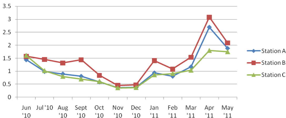
Fig. 7. Monthly Variation of Nitrate across the Sampling Stations in Lower River Benue
