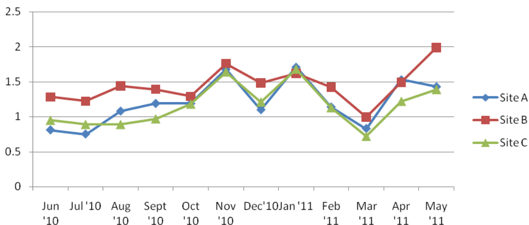
Fig. 8. Monthly Variation of Phosphate across the Sampling Stations in Lower River Benue
