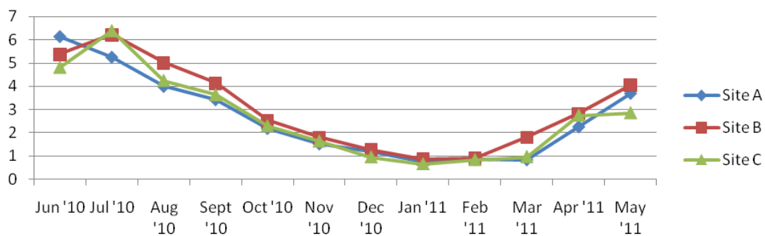
Fig. 4. Monthly Variation of Turbidity across the Sampling sites in Lower River Benue
