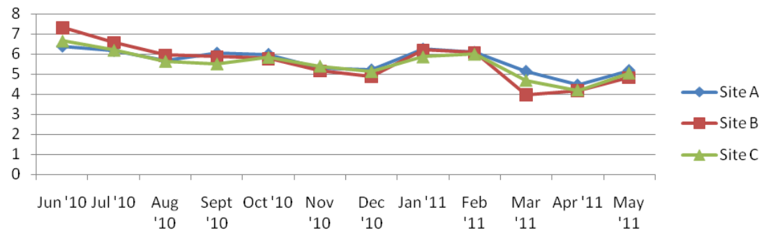
Fig. 5. Monthly Variation of Dissolved Oxygen across the Sampling sites in Lower River Benue
