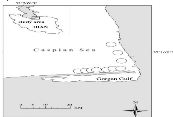
Fig. 1. Location of study and sampling positions in Caspian Sea, Circles showed sampling study area
